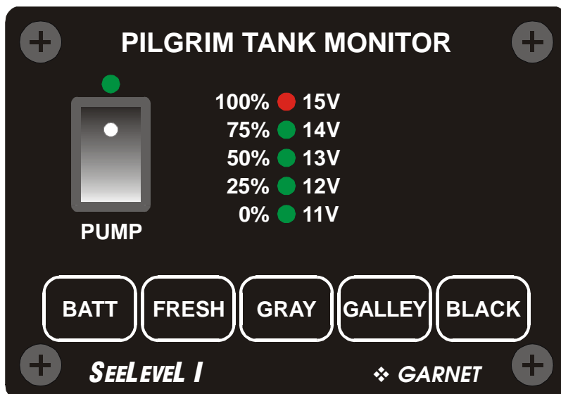
Four tank model
